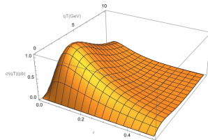
Figure 3: At 100 GeV and \lambda_1 = \lambda_2 = \lambda_3 = 0.1
