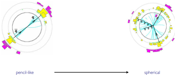
Figure 1: \tau from 0 to 1/2
