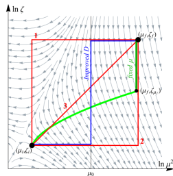
Figure 2: Null Evolution curve
